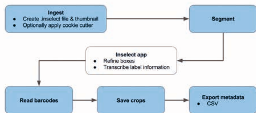
Figure 4. A typical Insect workflow. Each of the blue boxes has a corresponding command-line tool that operates on batches of images.
